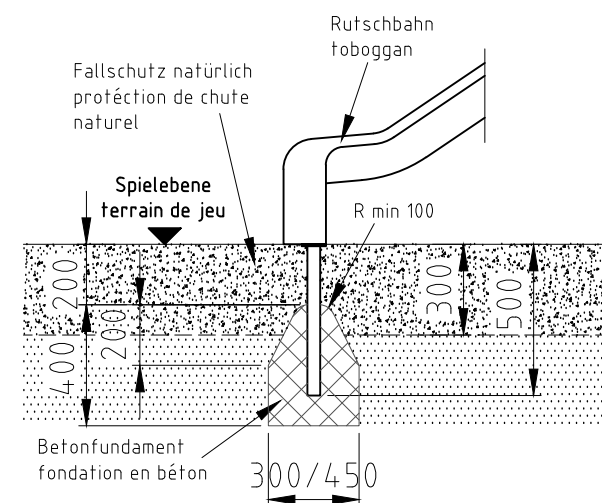
Fundament F09
