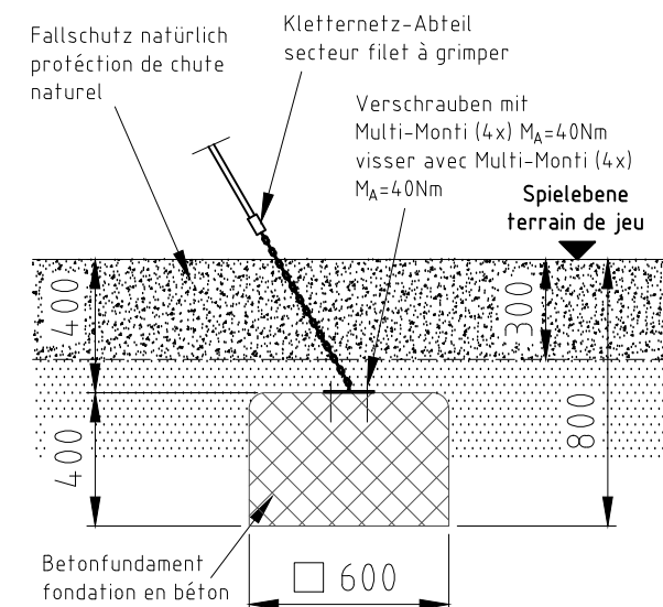
Fundament F08
